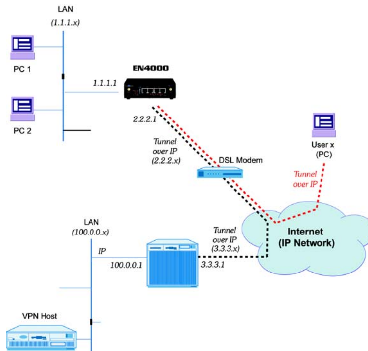
Figure 9-18. EN-4000 Tunnel Switching between VPN Client and VPN Host
