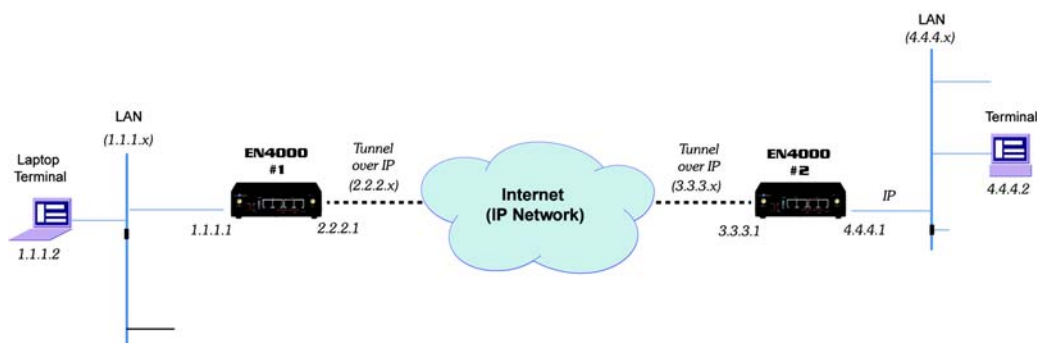
Figure 9-15. EN-4000s as VPN Gateways
