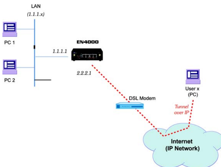
Figure 9-17. EN-4000 Terminating Tunnel from VPN Client
