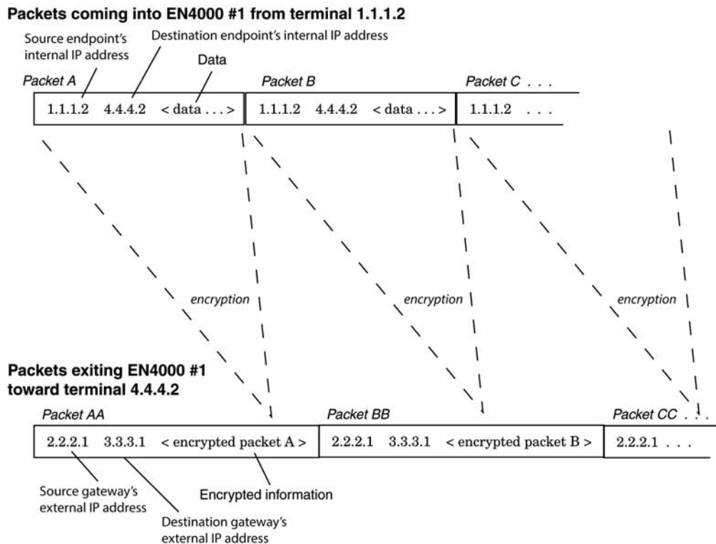
Figure 9-16. Sample IPsec Encryption and Encapsulation
